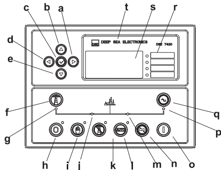
Control module
